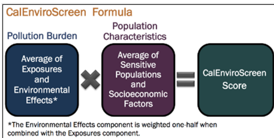
Figure 8-4: CalEnviroScreen Formula
